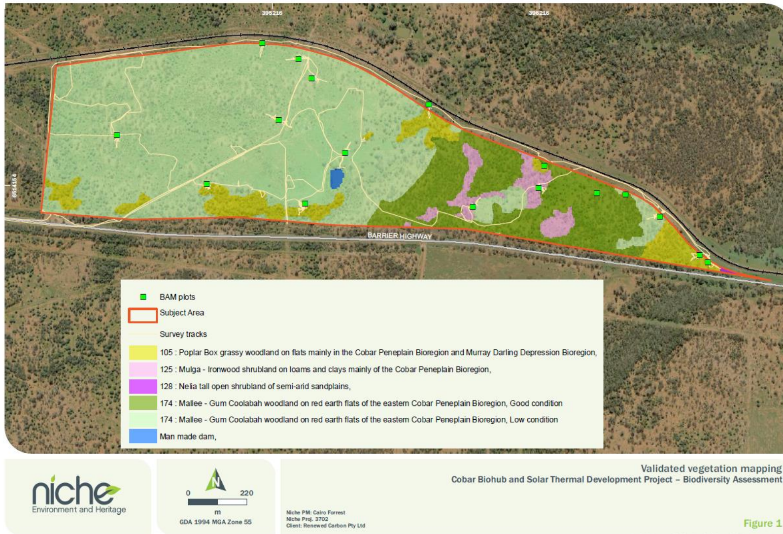
Figure 7-1 Vegetation mapping for the Site
